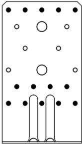
Nailing pattern 5
