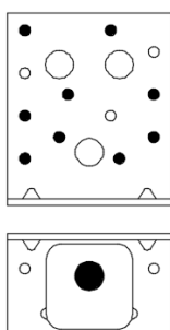
Nailing pattern 7
