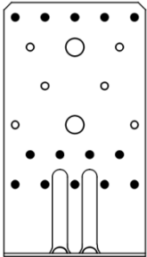
Nailing pattern 2
