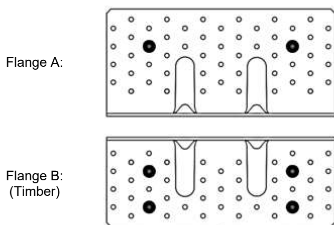
Nailing pattern 10
