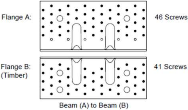
Nailing pattern 5
