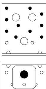
Nailing pattern 8
