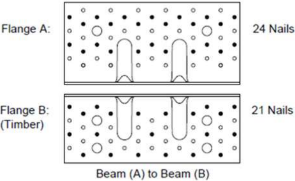
Nailing pattern 4
