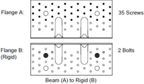
Nailing pattern 9
