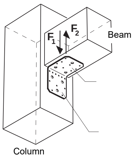
Figure C2-2-2: Beam to column connection – Angle bracket without a rib
