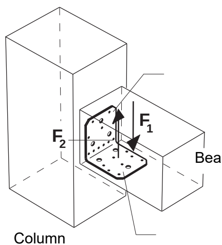
Figure C2-2-2: Beam to column connection – Angle bracket without a rib
