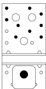
Nailing pattern 6
