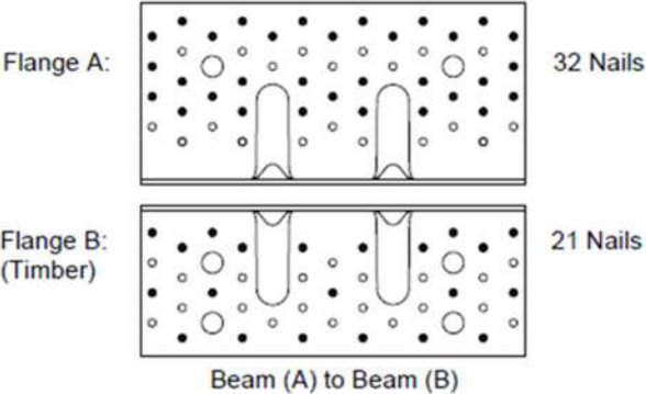
Nailing pattern 6
