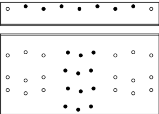
Timber to timber
