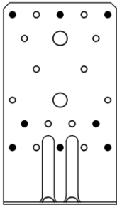
Nailing pattern 4
