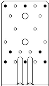
Nailing pattern 1
