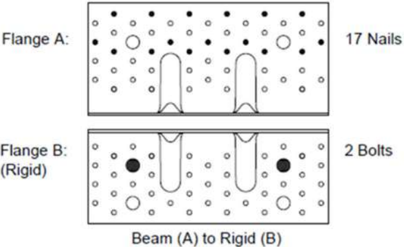
Nailing pattern 8
