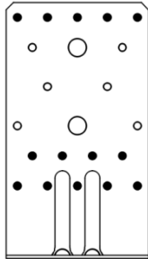
Nailing pattern 3
