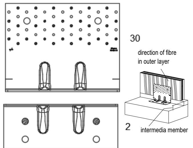
Nailing pattern 8
