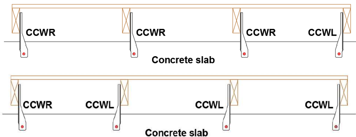
Figure 6: CCW arrangement
