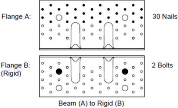
Nailing pattern 7
