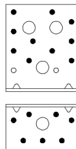
Nailing pattern 5
